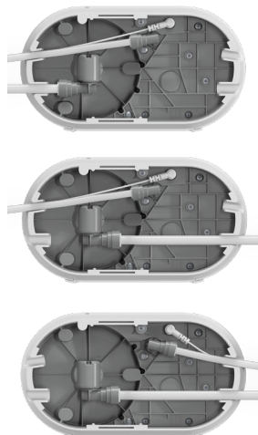
Bottom of unit: Tubing can be installed multiple ways to maximize your installation options.
